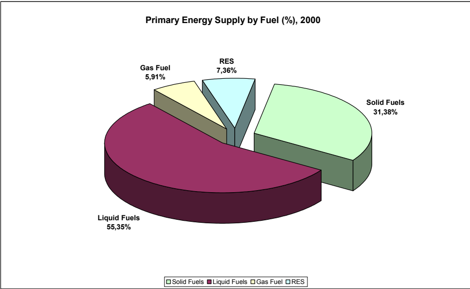
Chart 1. Percentage of primary energy supply by fuel in 2000
