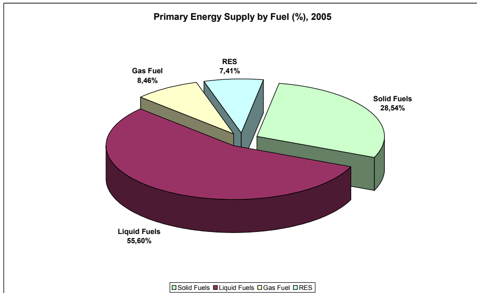
Chart 3. Percentage of primary energy supply by fuel in 2005 (projection)
