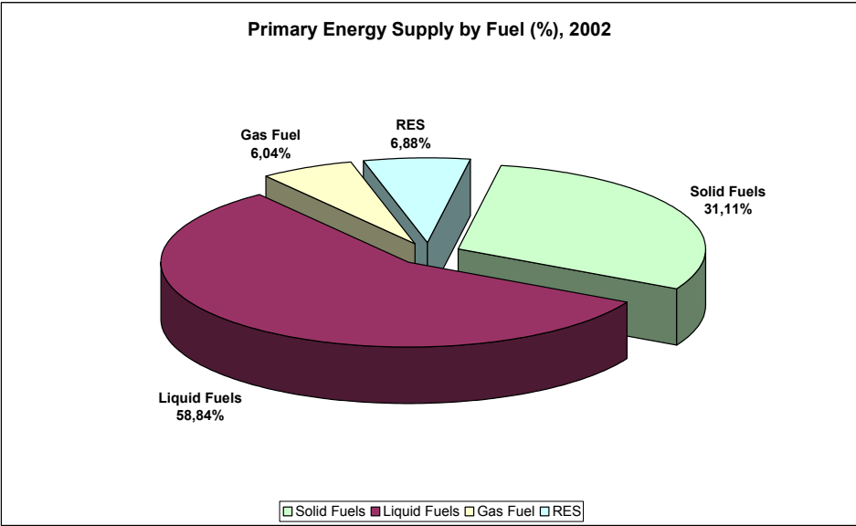
Chart 2. Percentage of primary energy supply by fuel in 2002
