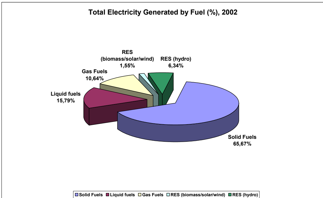
Chart 5. Percentage of total electricity generation, by fuel in 2002
