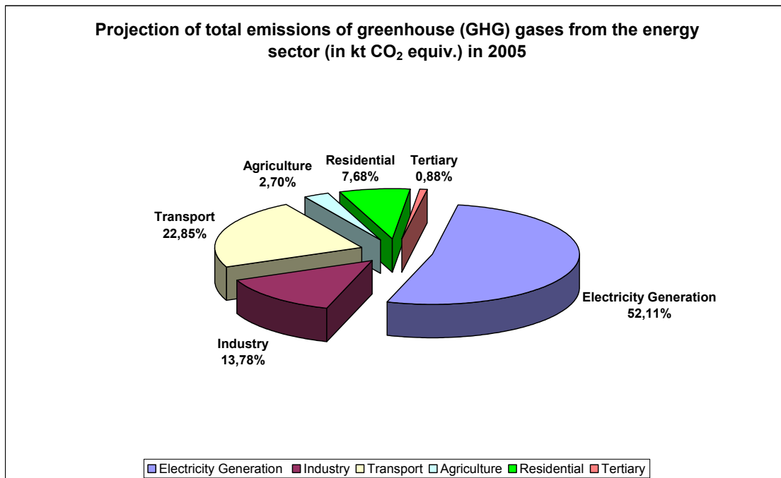
Chart 7. Projected percentage of total emissions of greenhouse gases by sector in 2005
