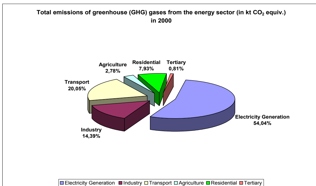
Chart 6. Percentage of total emissions of greenhouse gases by sector in 2000
