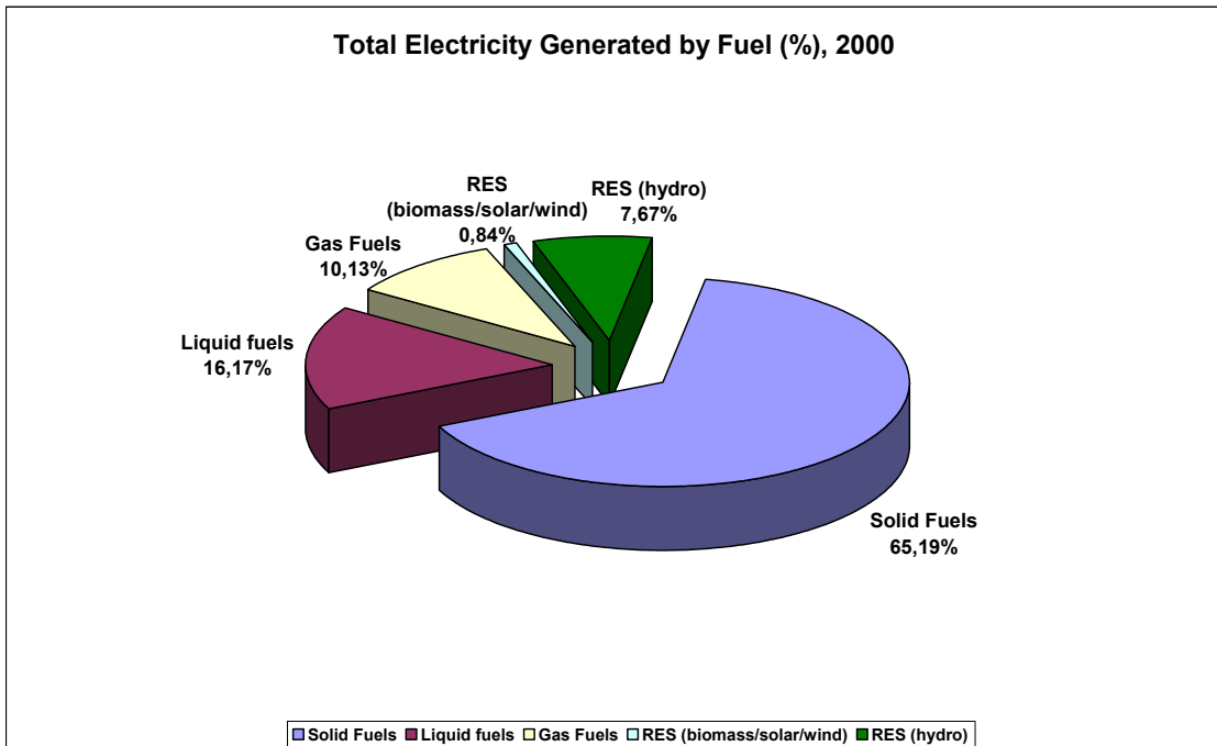
Chart 4. Percentage of total electricity generation, by fuel in 2000
